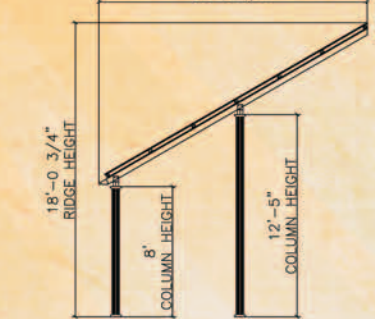
PVL-C18HP 6 - Solar Panels
