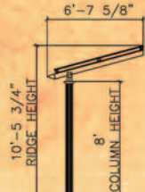
PVL-C6 2 - Solar Panels
