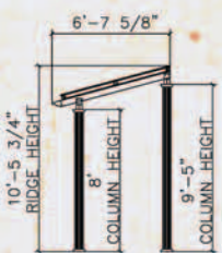
PVL-SP6 2 - Solar Panels
