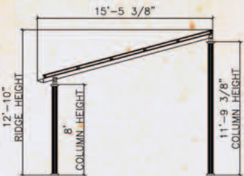
PVL-SP15 5 - Solar Panels
