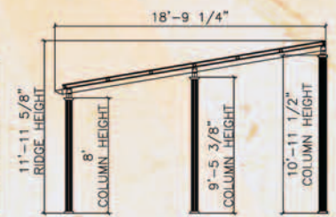
PVL-SP18LP 6 - Solar Panels
