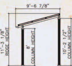
PVL-SP9 3 - Solar Panels
