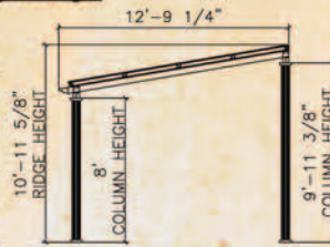
PVL-SP12LP 4 - Solar Panels
