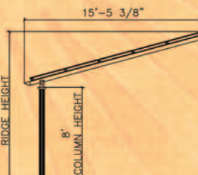
PVL-C15 5 - Solar Panels
