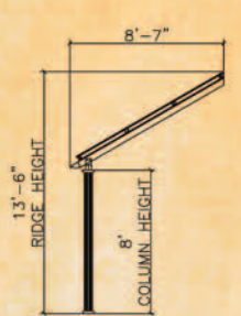
PVL-C8HP 3 - Solar Panels
