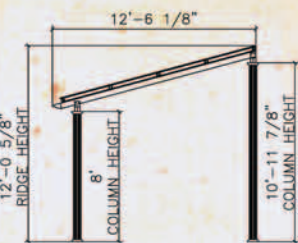
PVL-SP12 4 - Solar Panels
