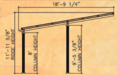
PVL-C18LP 6 - Solar Panels
