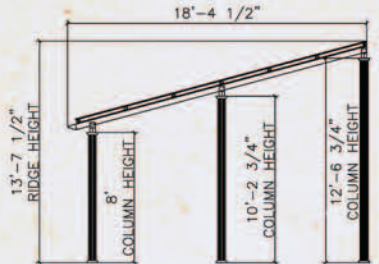
PVL-SP18 6 - Solar Panels
