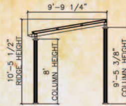
PVL-SP9LP 3 - Solar Panels
