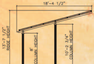
PVL-C18 6 - Solar Panels
