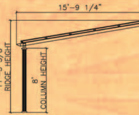
PVL-C15LP 5 - Solar Panels
