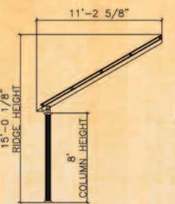
PVL-C11HP 4 - Solar Panels
