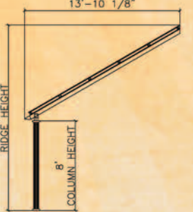
PVL-C13HP 5 - Solar Panels
